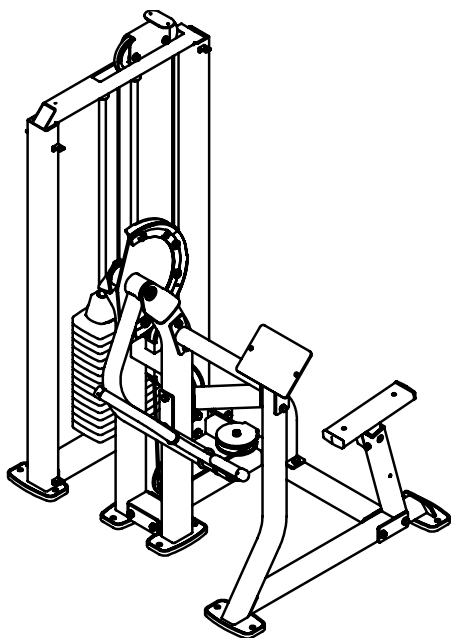
Above shows Step 5 assembled and completed.
