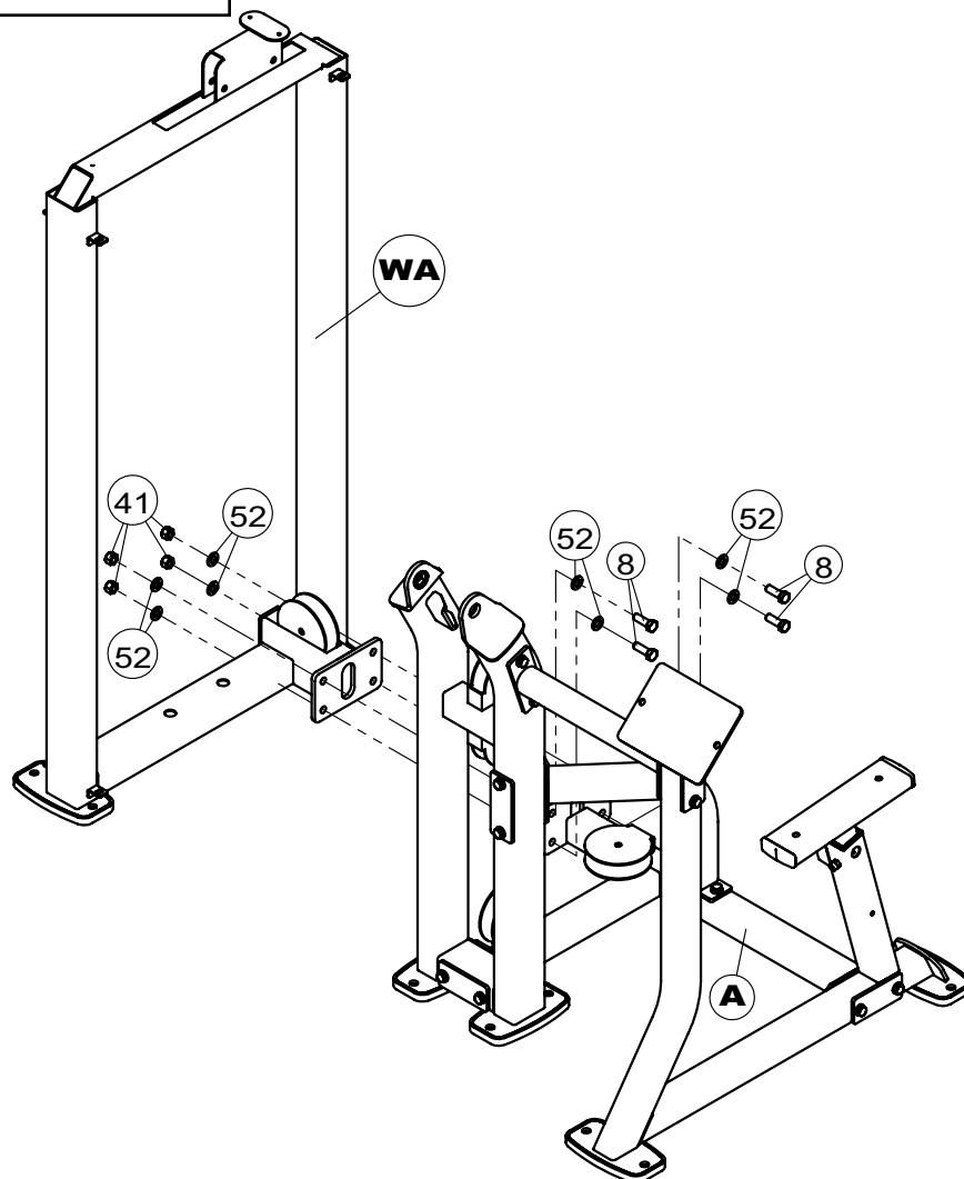
Above shows Step 2 assembled and completed.
