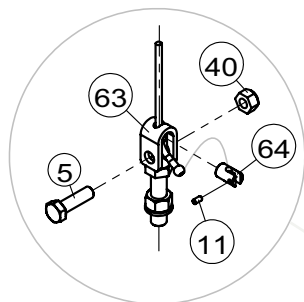
Above shows Step 5 assembled and completed.
