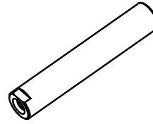
PART #66-SHAFT PIN, 1PCS. Φ25.4X137mm
