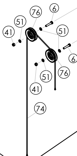
Above shows Step 6 assembled and completed.
