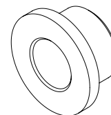
PART #63 - BUSHING, 2PCS. Ø25xØ12.2x13mm
