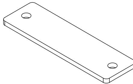
PART #77 - STEEL PLATE, 2PCS. 170x50x6mm
